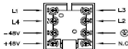
RACCORDEMENT CLIENT ISSUE 01
